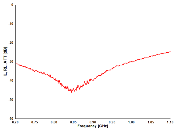
Return Loss (Port 4)
