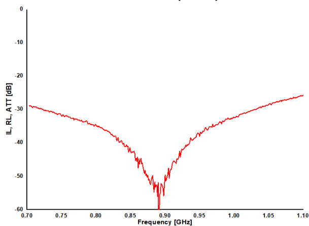
Return Loss (Port 2)
